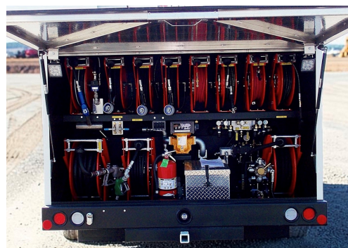
Reel bank - diesel, oils, grease & water hose stations.
