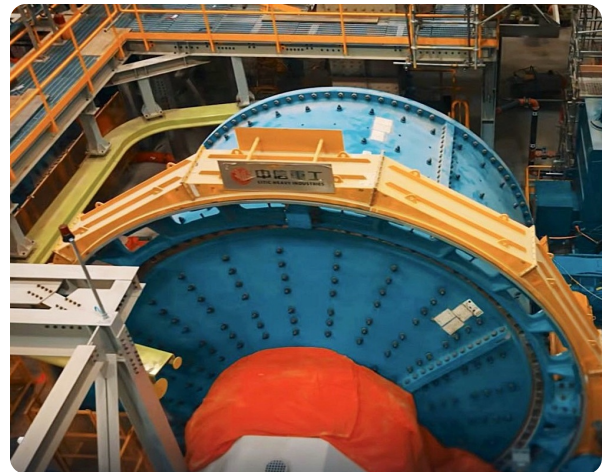
Relining bay fitted with monorail track for positioning the Bolt Buster.
