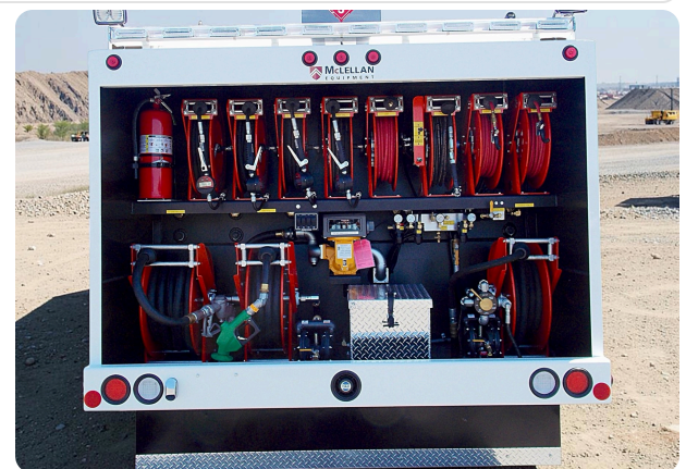
Rear reel bank: hydraulic-rewind hose reels and meter/gauge panel.
