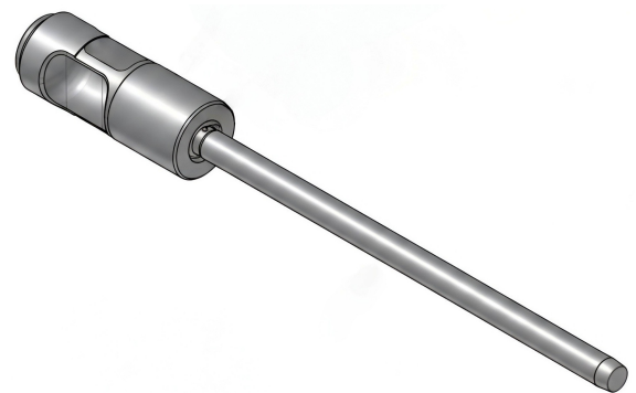
Moil rod and handle assembly.
