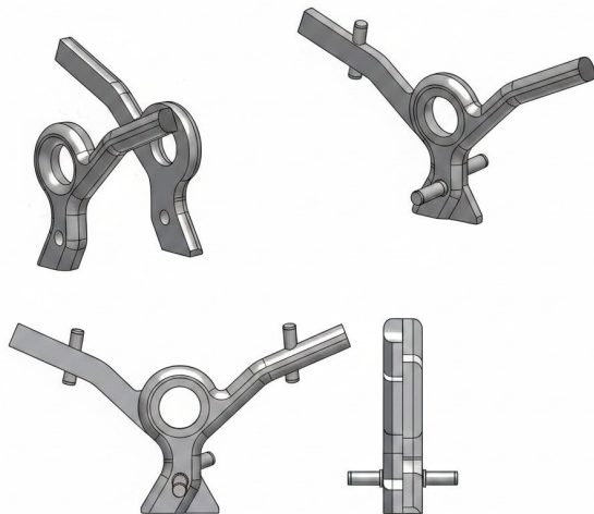
Liner lifting scissors assembly, multiple views.
